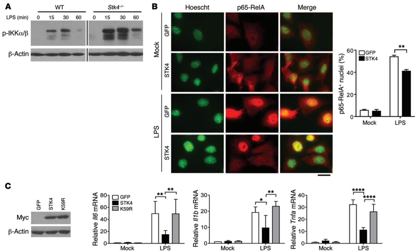
Figure 3. STK4 kinase activity is critical to inhibit TLR4/NF-κB activation. (A) The levels of phosphorylated IKKα/β in LPS-stimulated WT and Stk4 -/- BMMs were detected by immunoblotting analysis. Samples were run on the same gel but not contiguous, as indicated by the black line. (B) Primary MEF cells overexpressing GFP or STK4 were treated with or without LPS, followed by immunostaining with Hoechst and anti-p65-RelA (scale bar: 20 μm, representative images). The number of p65-RelA + nuclei was counted from >50 cells (mean ± SD using 2-tailed, unpaired Student’s t test). (C) Primary MEFs overexpressing GFP, STK4, or the K59R mutant were stimulated with LPS to detect mRNA levels of Il6 , Il1b , and Tnfa . Values were normalized for β-actin mRNA levels (mean ± SD, n = 4, 2-way ANOVA with Holm-Sidak’s multiple comparisons test). * P < 0.05, ** P < 0.01, and **** P < 0.0001.
